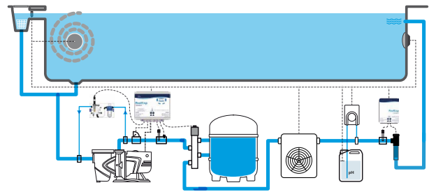
TYPICAL ELECTROLYSIS INSTALLATION
