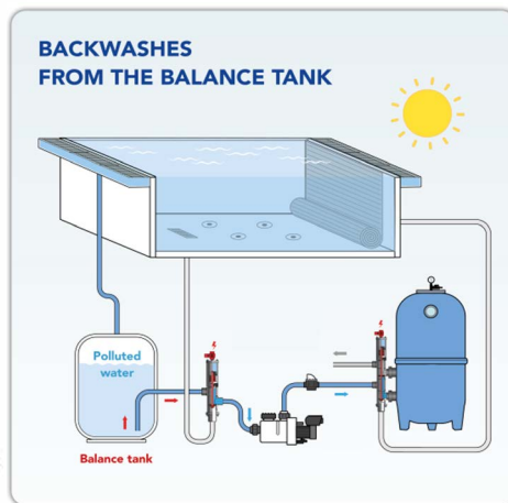
BACKWASH VIA MAIN DRAIN OR SKIMMER / BUFFER TANK
